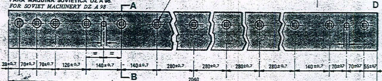
DETALLE D DETAIL D
